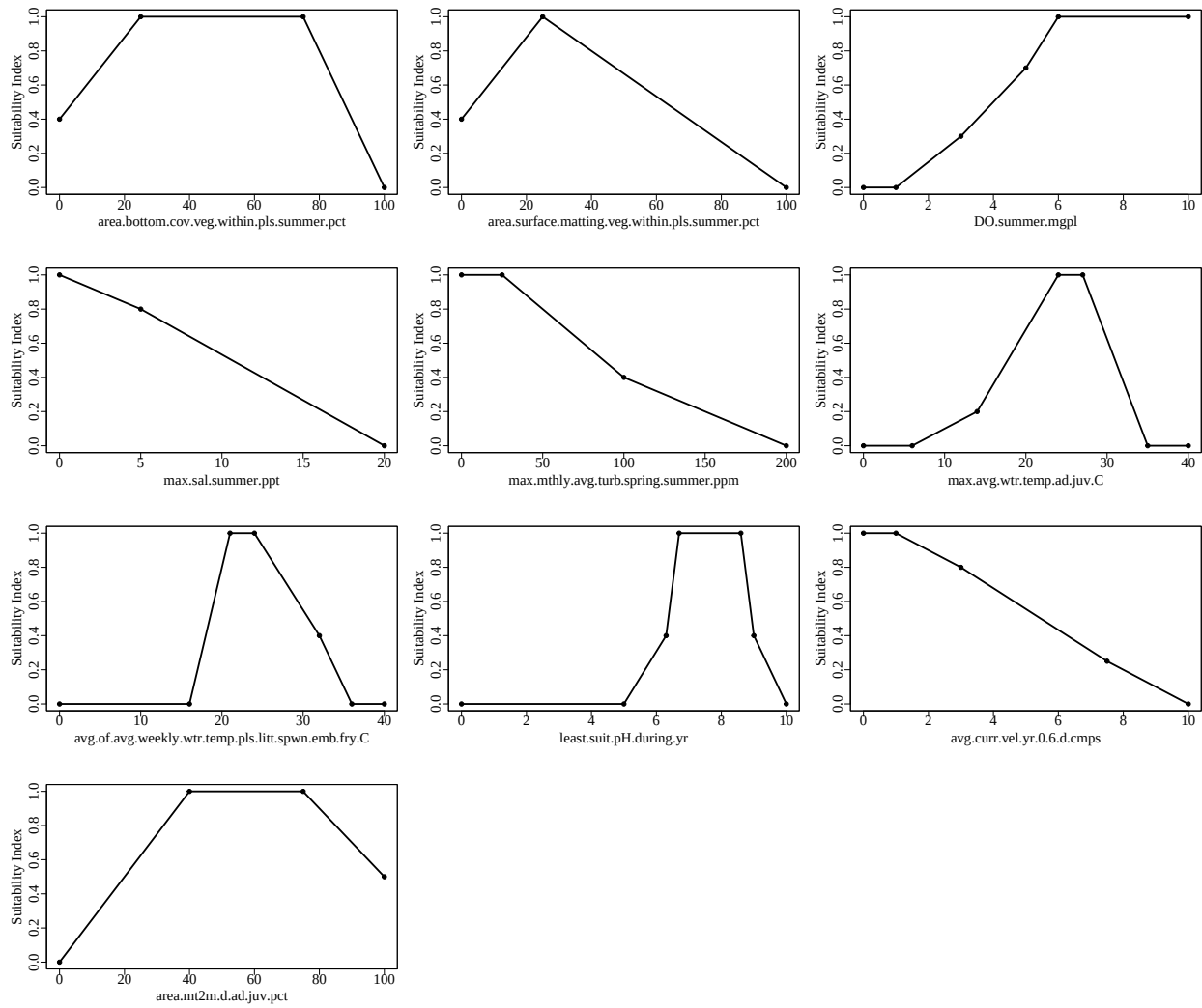
Figure 1. Suitability index graphs for variables included in the redearsunfishRiv model in ecorest.
